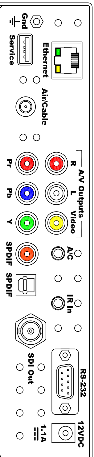
REAR VIEW
